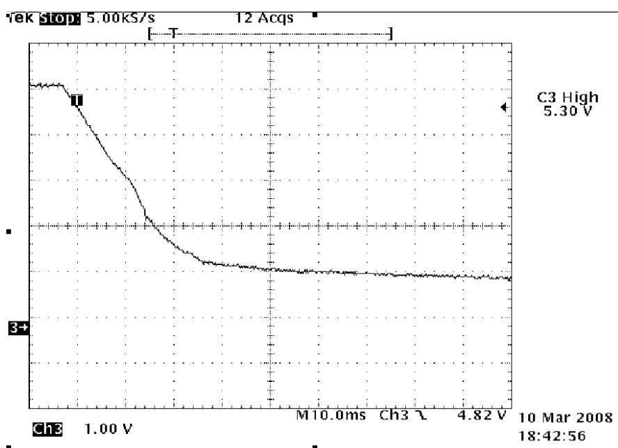
Figure 5. Pin8, U30. Umbilical Power ON->Power OFF, Battery is Off
